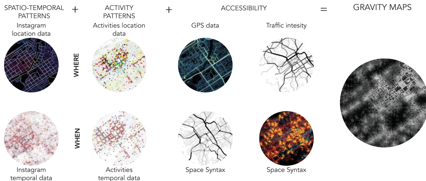
Figure 62. Scheme of the model used to draw up the gravity maps
